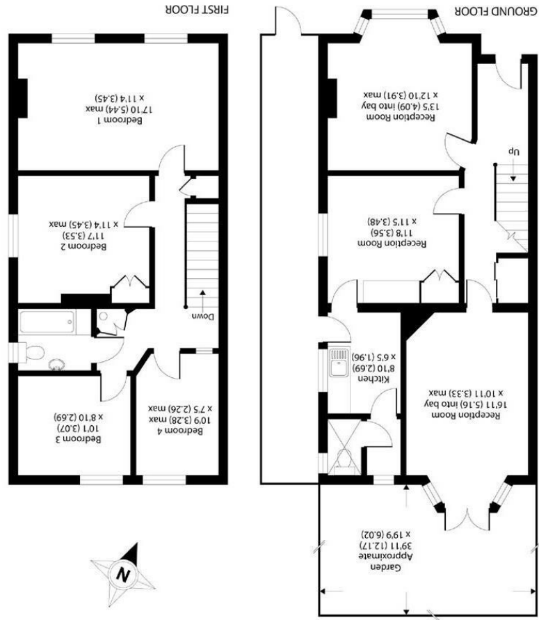
APPROX. GROSS INTERNAL FLOOR AREA 1391 SQ FT 129.2 SQ METRES
